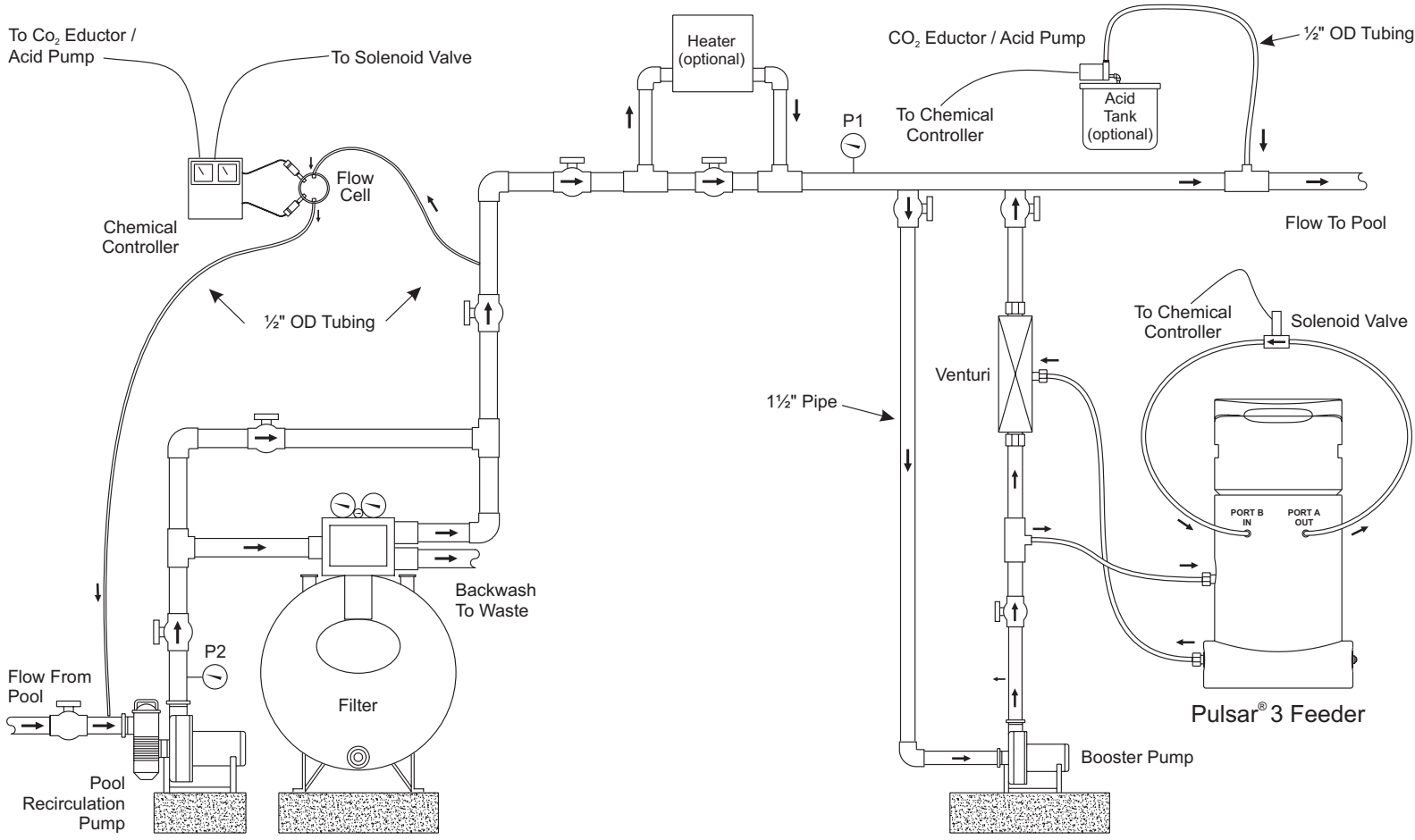
Pulsar ® 3 Installation Schematic Layout 3/4 HP Pump & Venturi Installation 09-22-06 Standard Installation
