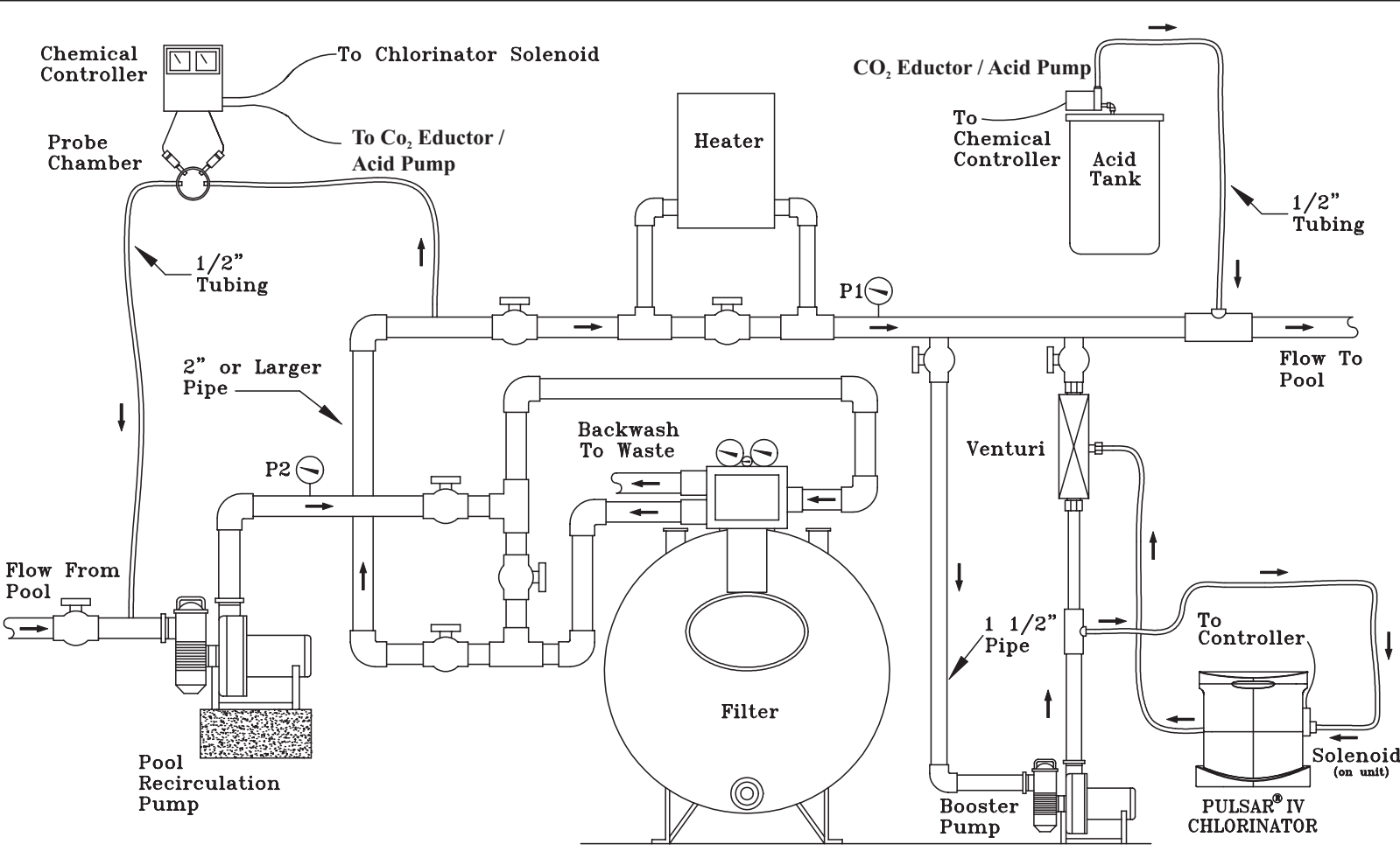
PULSAR ® IV Installation Schematic Layout 1 HP Pump & Venturi Installation 09/06 Standard Installation
